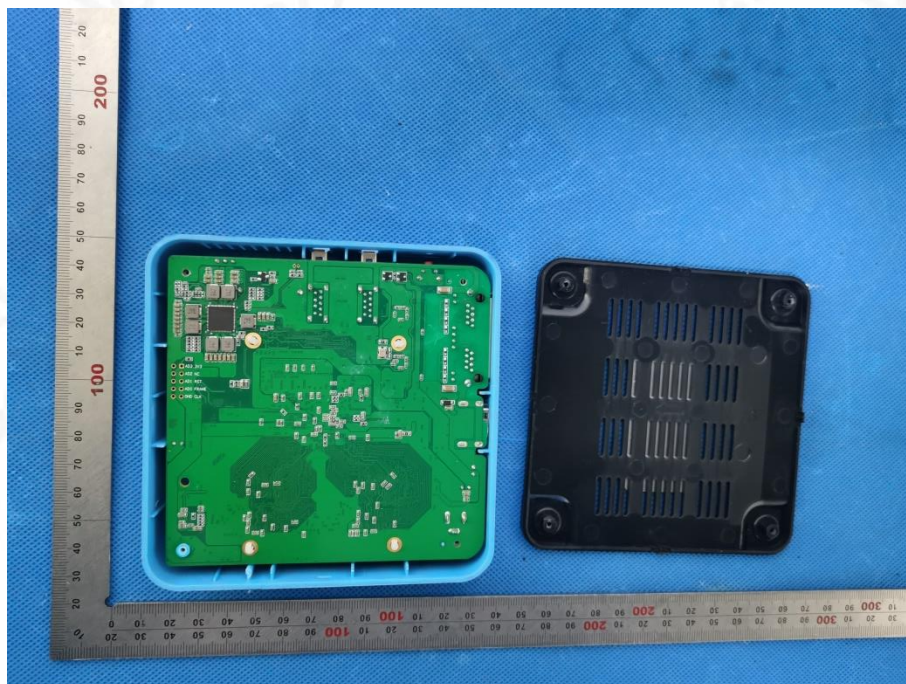
Fig. 6 –Internal view
