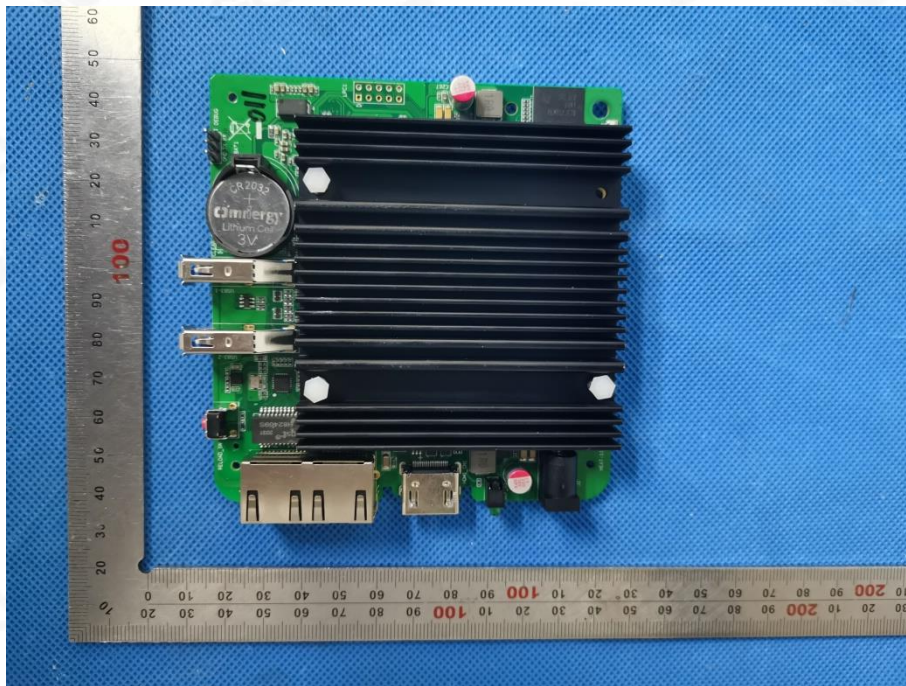
Fig. 7 –PCB view
